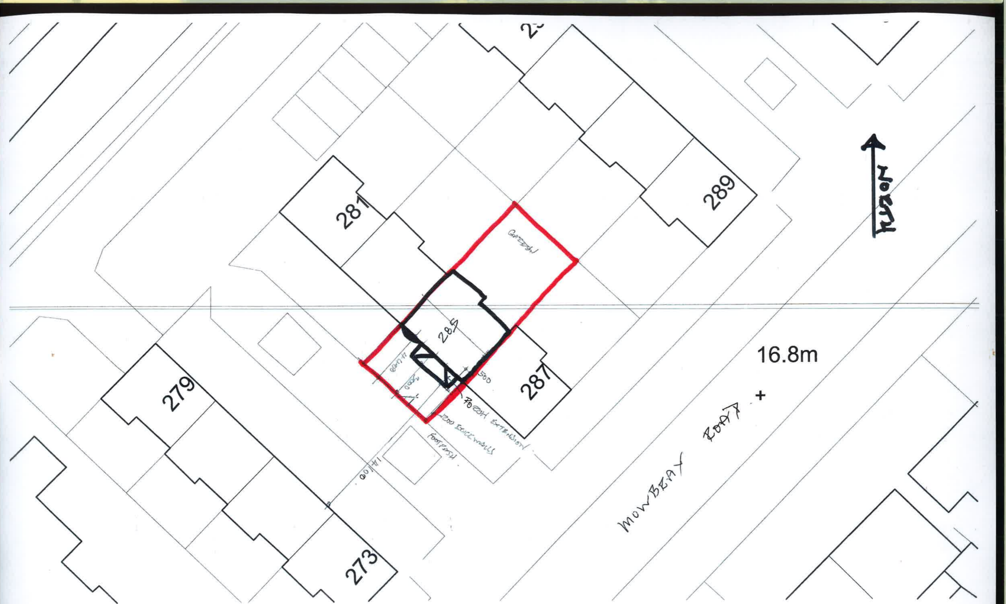
PROPOSED BLOCK PLAN. 1:200.
